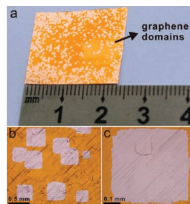
Figure 1. (a) Photo of the as-grown, separated graphene domains on Cu foil. (b, c) Optical microscopy images of the graphene domains in (a). The parallel dark stripes correspond to surface unevenness induced by mechanical processing of Cu foil.
